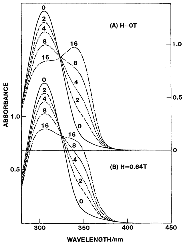
Fig. 1. Photoreaction of 1 ( 12 ) in benzene as detected by UV-absorption spectroscopy (A) in the absence and (B) in the presence of an external magnetic field (0.64 T). The numerals attached to the curves refer to the irradiation time in minute. Excitation source; 500-W Xe arc with combined color glass filters (Toshiba UV-D33S, UV-25, and UV-33).
